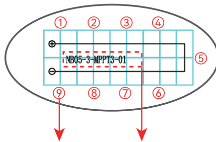
PV Array Wiring Diagram
