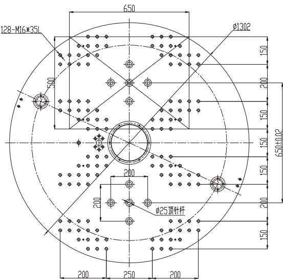
圆盘/Rotary Table
