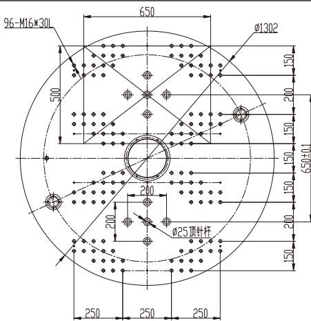
圆盘/Rotary Table
