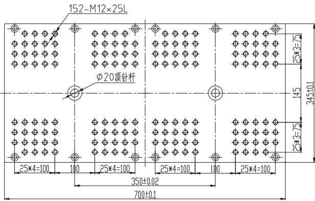
双滑板/Double Slide
