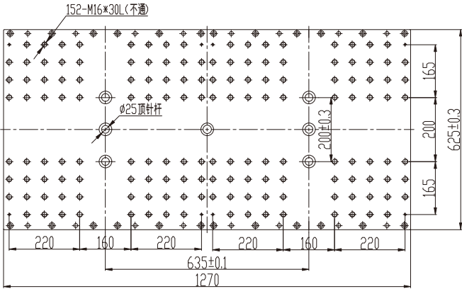
双滑板/Double Slide
