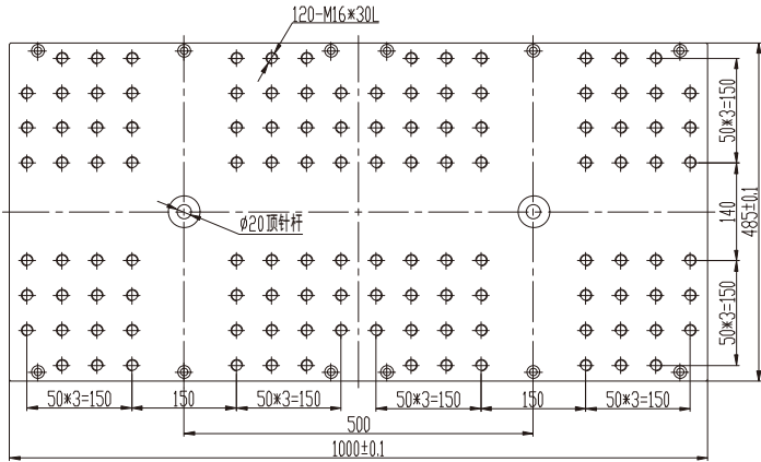
双滑板/Double Slide
