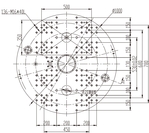
圆盘/Rotary Table
