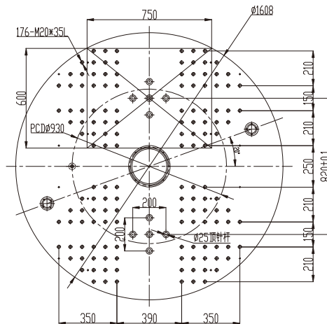
圆盘/Rotary Table
