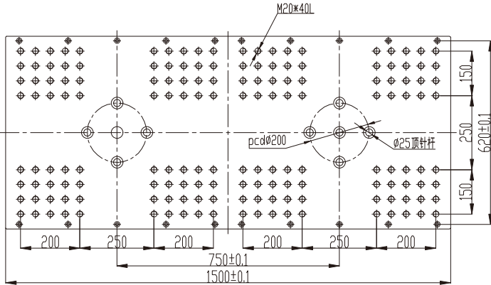
双滑板/Double Slide
