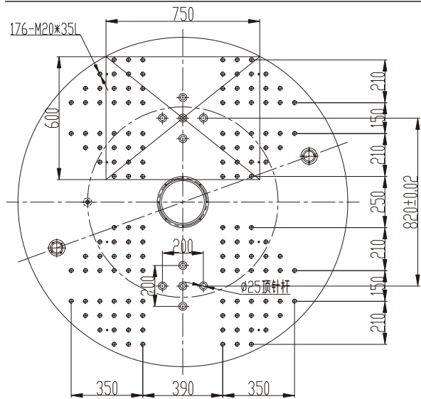
圆盘/Rotary Table
