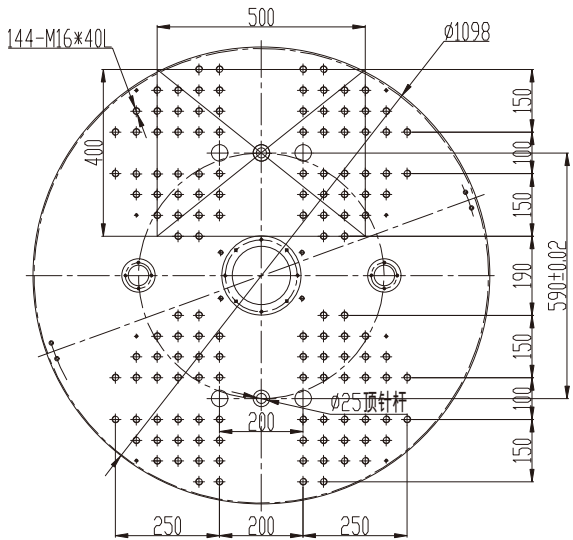
圆盘/Rotary Table
