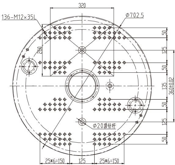
圆盘/Rotary Table
