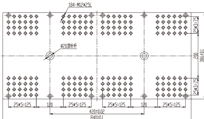
双滑板/Double Slide
