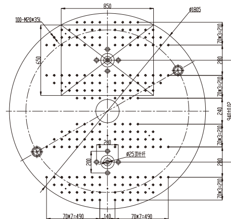
圆盘/Rotary Table
